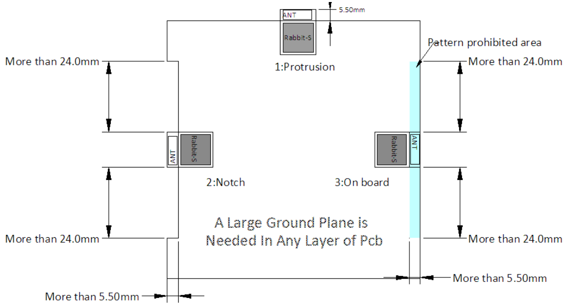
Figure 3: Module Placement
