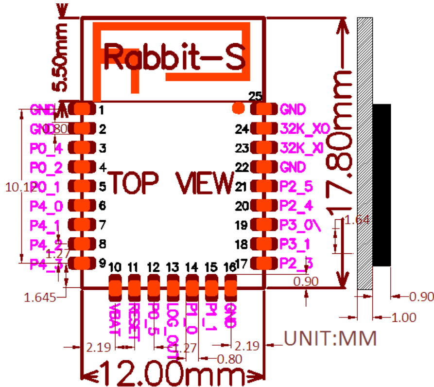
Figure 2: Mechanical Information
