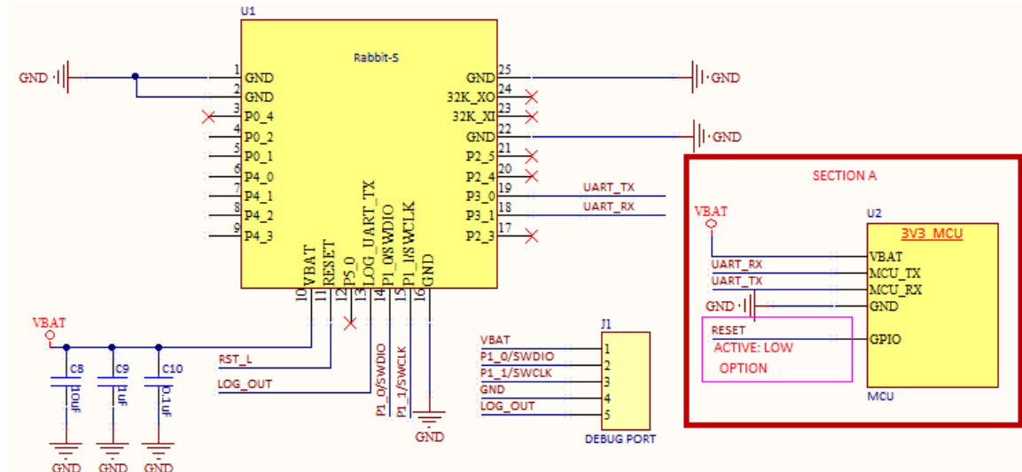
Figure 1: Module Reference Design
